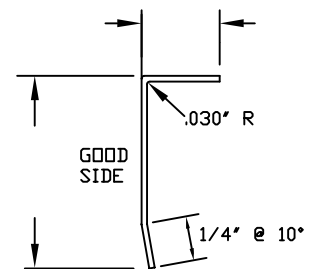
FLAT TRIM
