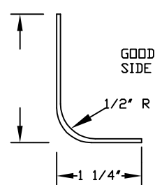
COVE BASE
